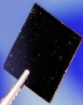
GRAPHEN
