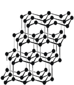
DIAMANT
