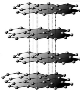
GRAPHIT
