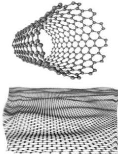
GRAPHEN
